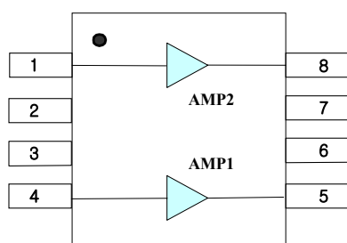
Block Diagram
