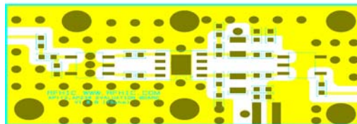
Evaluation Board Layout 5-200MHz
