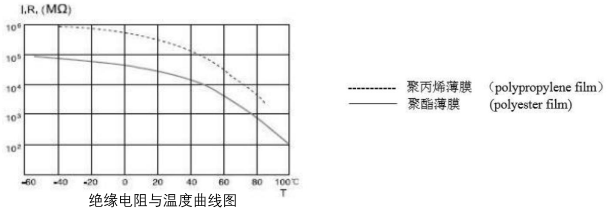
Insulation resistance and temperature curve
