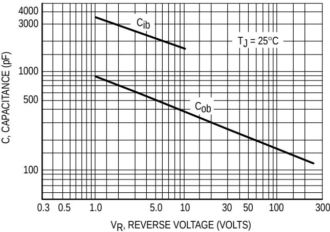
Figure 2. Capacitances
