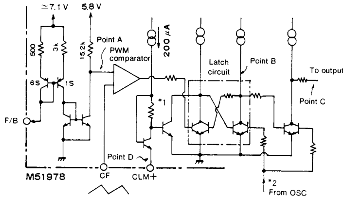
Fig.9 PWM comparator section, PWM latch and current limit latch section
