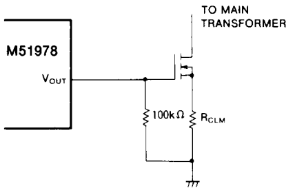
Fig. 33 Circuit diagram to prevent the MOS-FET gate potential rising
