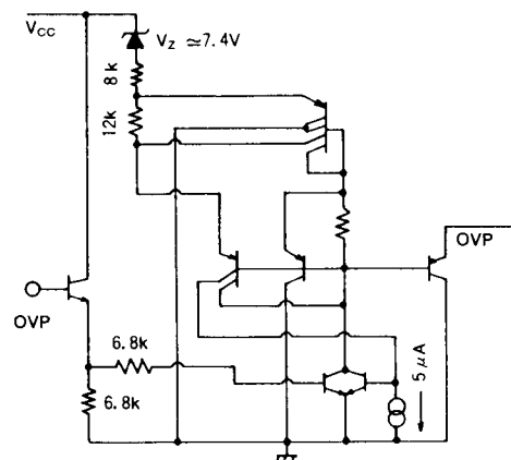
Fig.15 Detail diadram of OVP circuit
