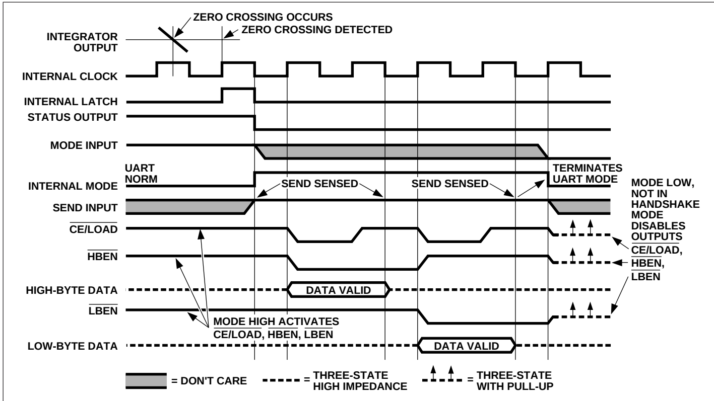
Figure 7. TC7109A Handshake With SEND INPUT Held Positive
