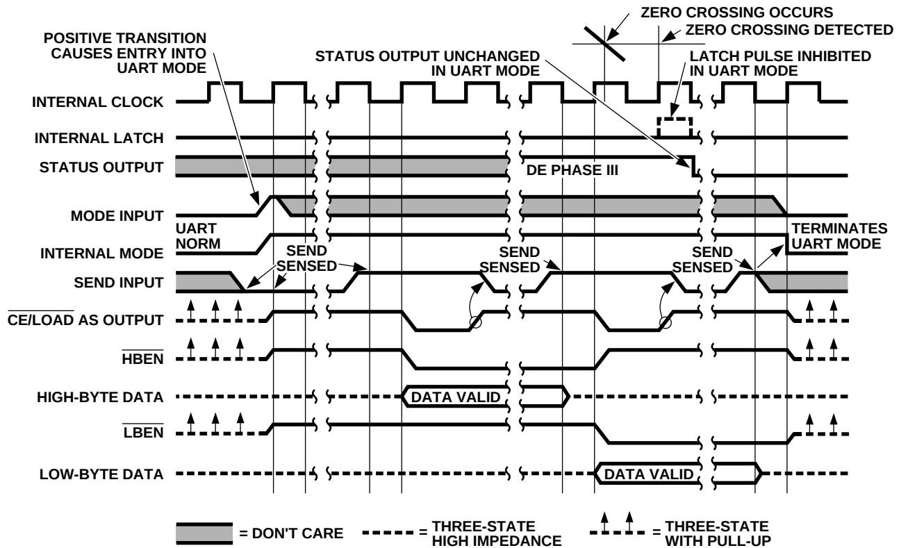
Figure 9. TC7109A Handshake Triggered by MODE Input
