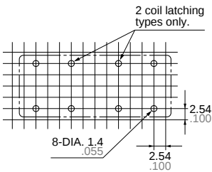
PC board pattern (Copper-side view)
