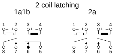
(Reset condition)
