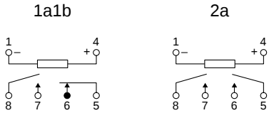
(Deenergized condition)
