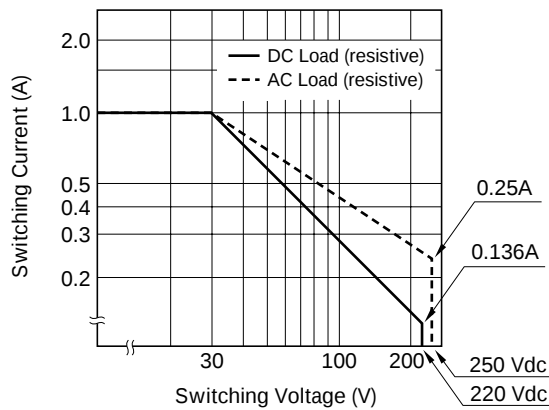
SWITCHING CAPACITY
