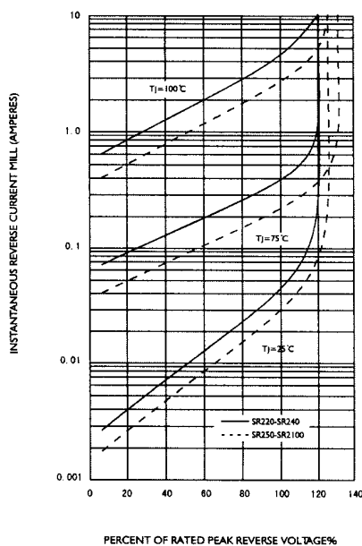
FIG.4-TYPICAL REVERSE CHARACTERISTICS
