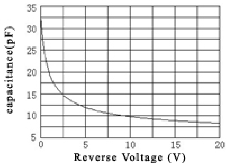
C-V Curve
